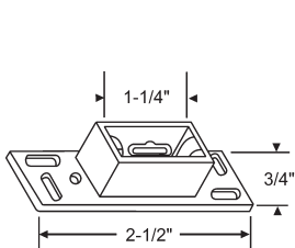
45-9 Drawer Mounting Bracket
