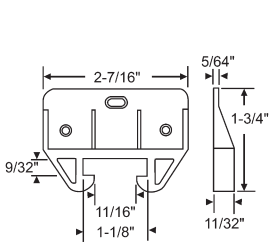
45-7 Drawer guide Old KD-07
