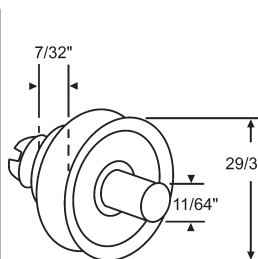
45-98 Drawer Roller with Axle
