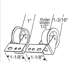
45-14 Drawer guide Old KD-14
