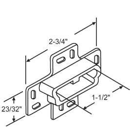
45-23 Drawer Mounting Bracket
